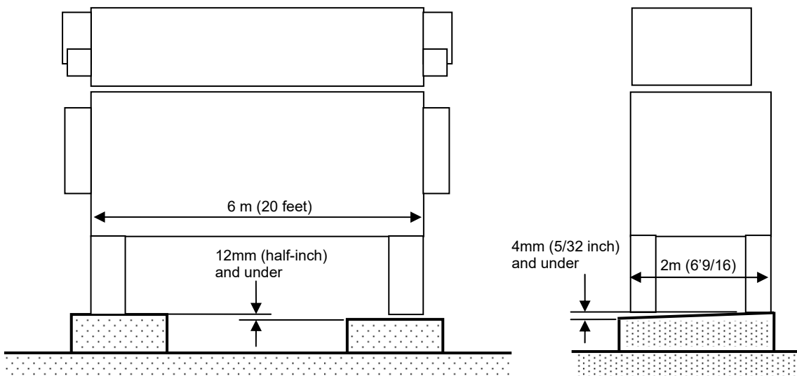
Permissible levelness for the absorption chiller installation
