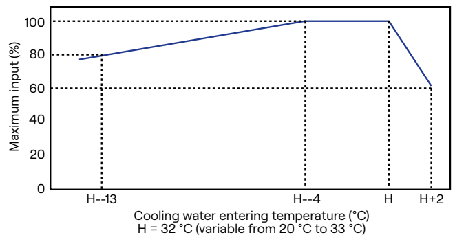
Graph 6 - Safe operating zone chart
