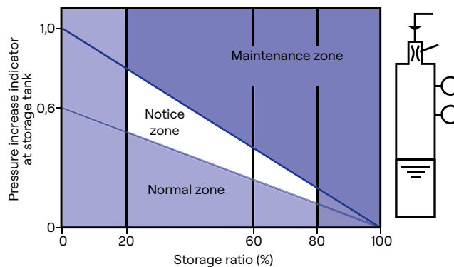
Graph 3 - Vacuum condition monitoring
