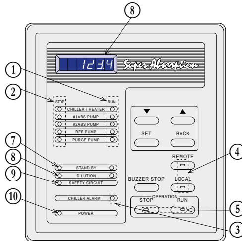
Display and control board Figure 2 - Indication lights
